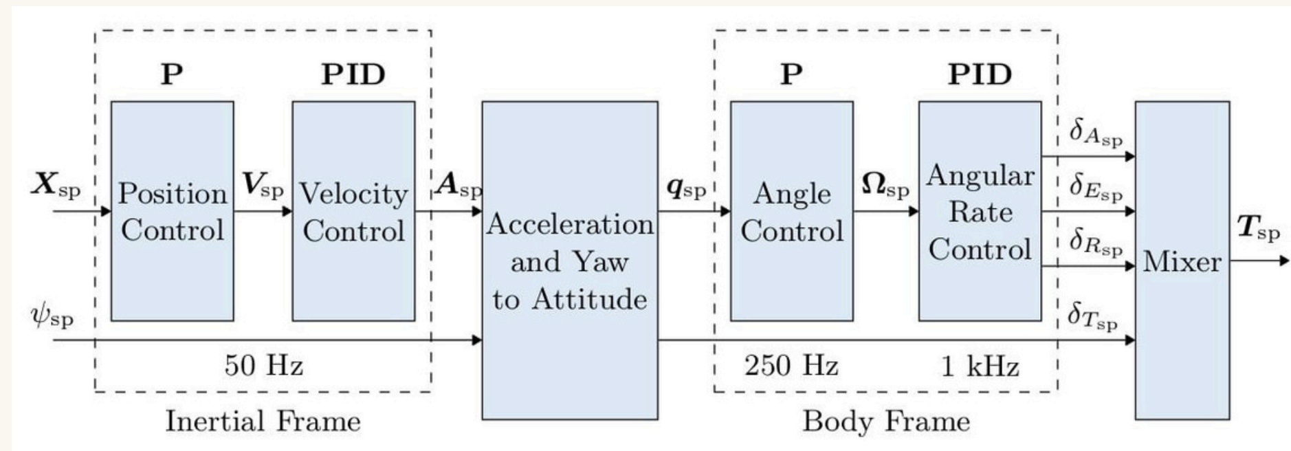
Cascaded PID
