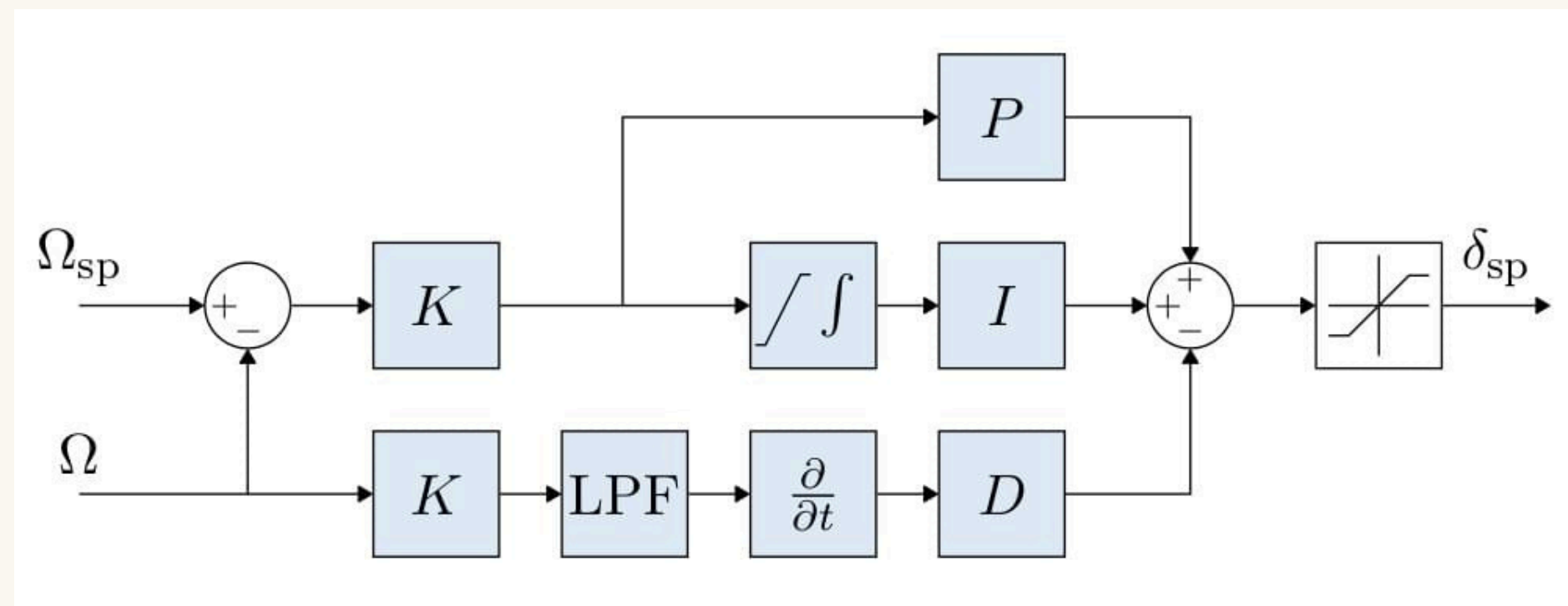
Individual PID loop
